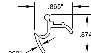
11 SASH BOTTOM LOCK RAIL 6063-T6 ALUMINUM
