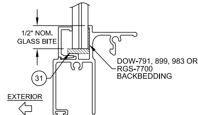
TYP. GLAZING DETAIL
